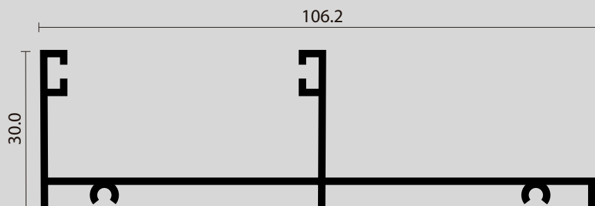
ALN702 JAMBA
