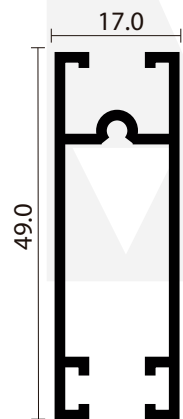
ALN390 HORIZONTAL INF.NAVE
